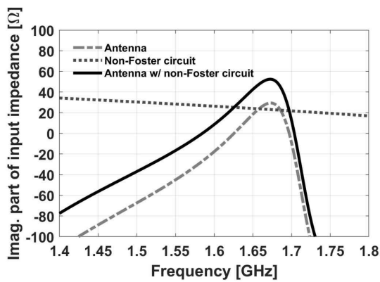
Fig. 5. Imaginary part of the input impedance
