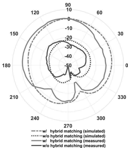
Fig. 10. Radiation patterns of the antenna
